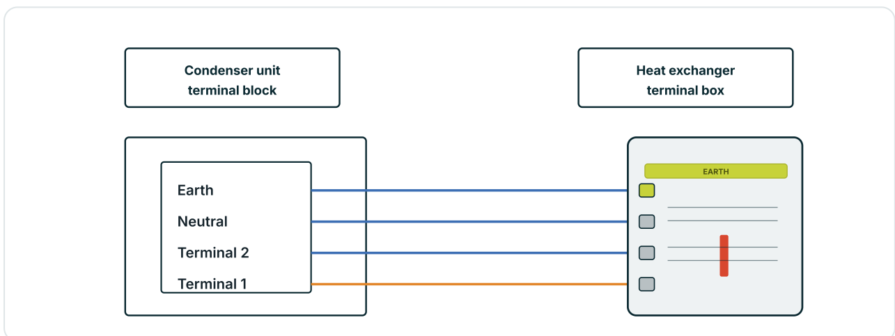
Electrical interconnection — the condenser unit terminal block (Earth, Neutral, Terminal 2, Terminal 1) wired across to the heat-exchanger terminal box.
